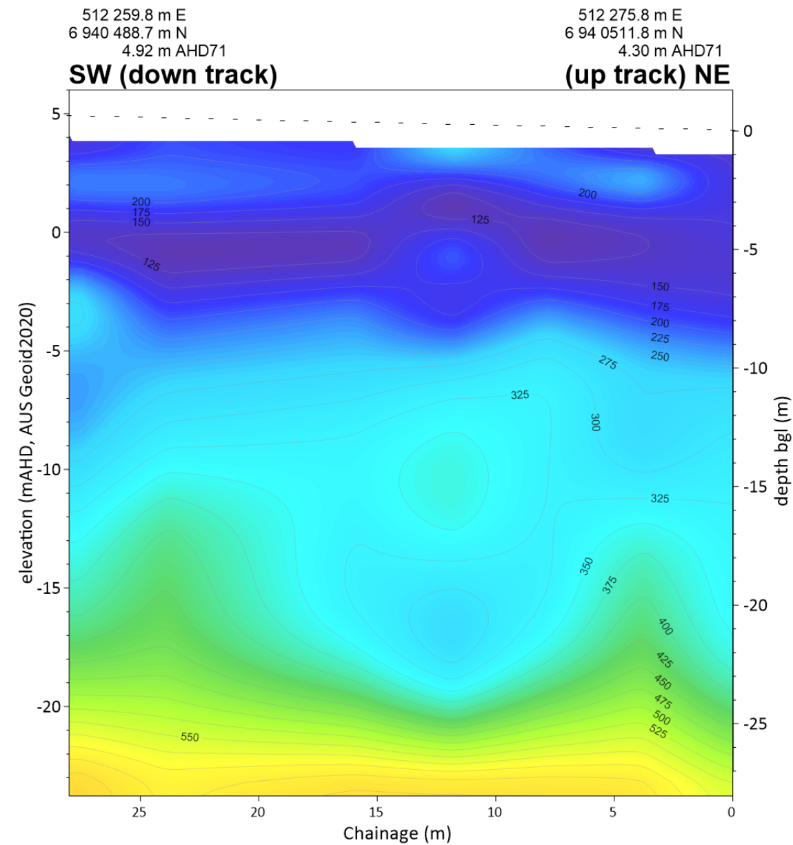
Seismic Line MASW AU-GP 147
